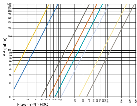
Pressure Drop
