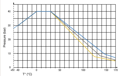
Pressure - Temperature
